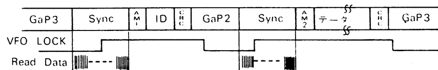
Fig. 2-20 Clock Pulse and VFO in Sync Zone
