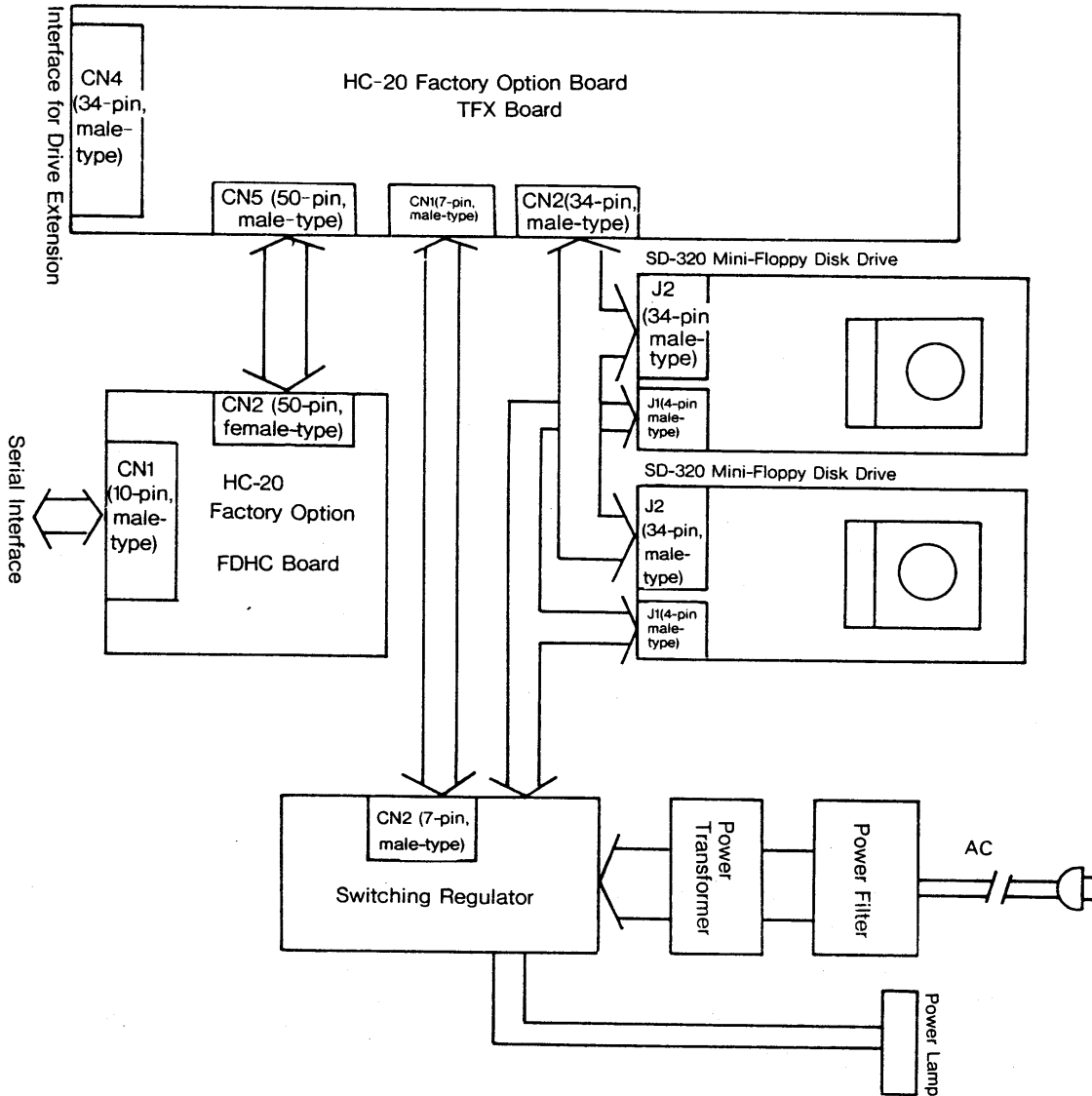
Fig. 2-1 BlockDiagram
