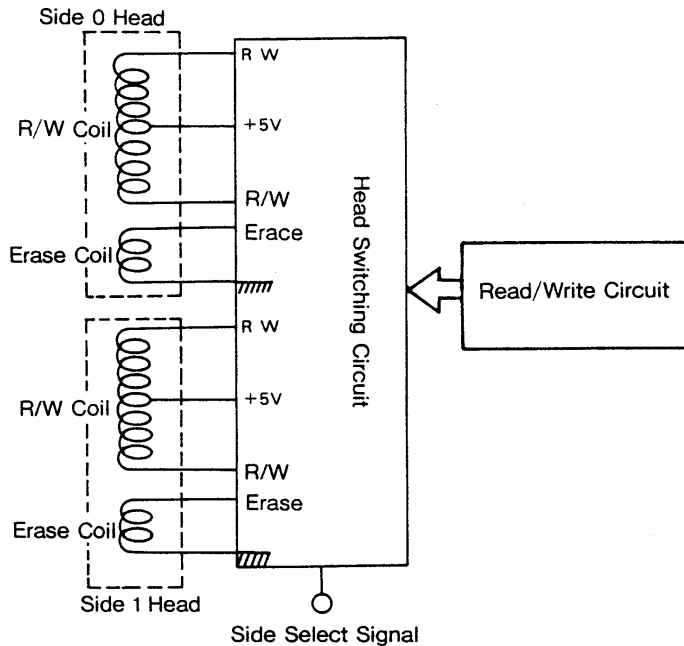
Fig. 2-12 Block Diagram of Magnetic Head
